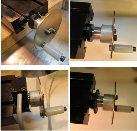
Fig.: Mounting the hand wheel. Design details may deviate from the images shown. Sherlines mill table is shown as well as Sherlines DRO (not included).
